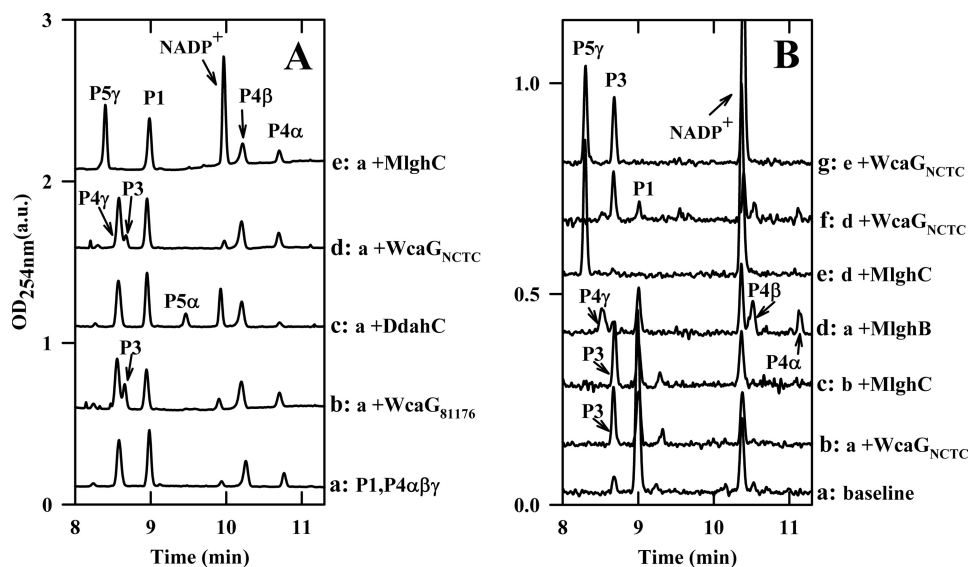
FIGURE 4. CE electropherograms highlighting the differences between the reductases WcaG NCTC and WcaG 81176 . The identity of all peaks is as described in Fig. 3. In addition, P3 is reduced GDP-6-deoxy- D -manno-heptose. Panel A , ~0.10 mM preformed P1, 7 \mu M MlghB, 0.10 mM NADPH, and 200 mM Tris-HCl, pH 8.0 were incubated at 37 °C for 15 min, and the reaction was filtered through a 10-kDa membrane to remove MlghB. The filtrate obtained comprised products P1, P4 \alpha , P4 \beta , and P4 \gamma in fixed proportions. It was incubated for 30 min at 37 °C as such ( trace a ) or supplemented with 3 \mu M concentrations each of the indicated enzymes. The data show that WcaG NCTC and WcaG 81176 have the same activity and cannot replace the reductase of their cognate pathway, MlghC or DdahC. Panel B , 6 \mu l of ~0.07 mM heptose and 3 \mu M DdahA ( trace a , base line) were supplemented with 3 \mu M concentrations of each of the indicated enzymes (without elimination of DdahA). The activity was recorded after 2.5 h incubation at 37 °C. The data show that the activity of MlghC is not affected by WcaG NCTC and vice versa. Integration data are provided in supplemental Table S2 .
