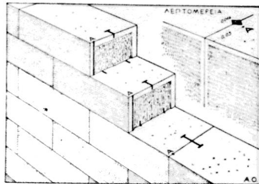
8 Setting blocks: anathyrosis, cuttings for clamps and dowels. Orlandos, Archaion Hellinon , Fig. 15
