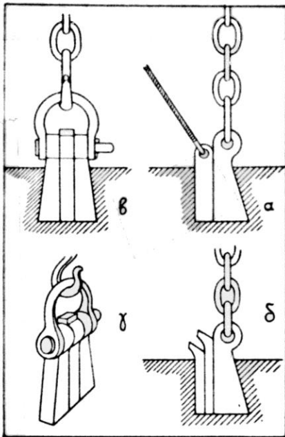
6 Types of lewis. Orlandos, Archaion Hellinon , Fig. 128.
