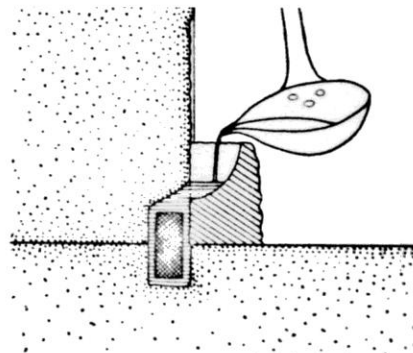
9 Pouring lead on dowel. Orlandos, Archaion Hellinon , Fig. 14.
