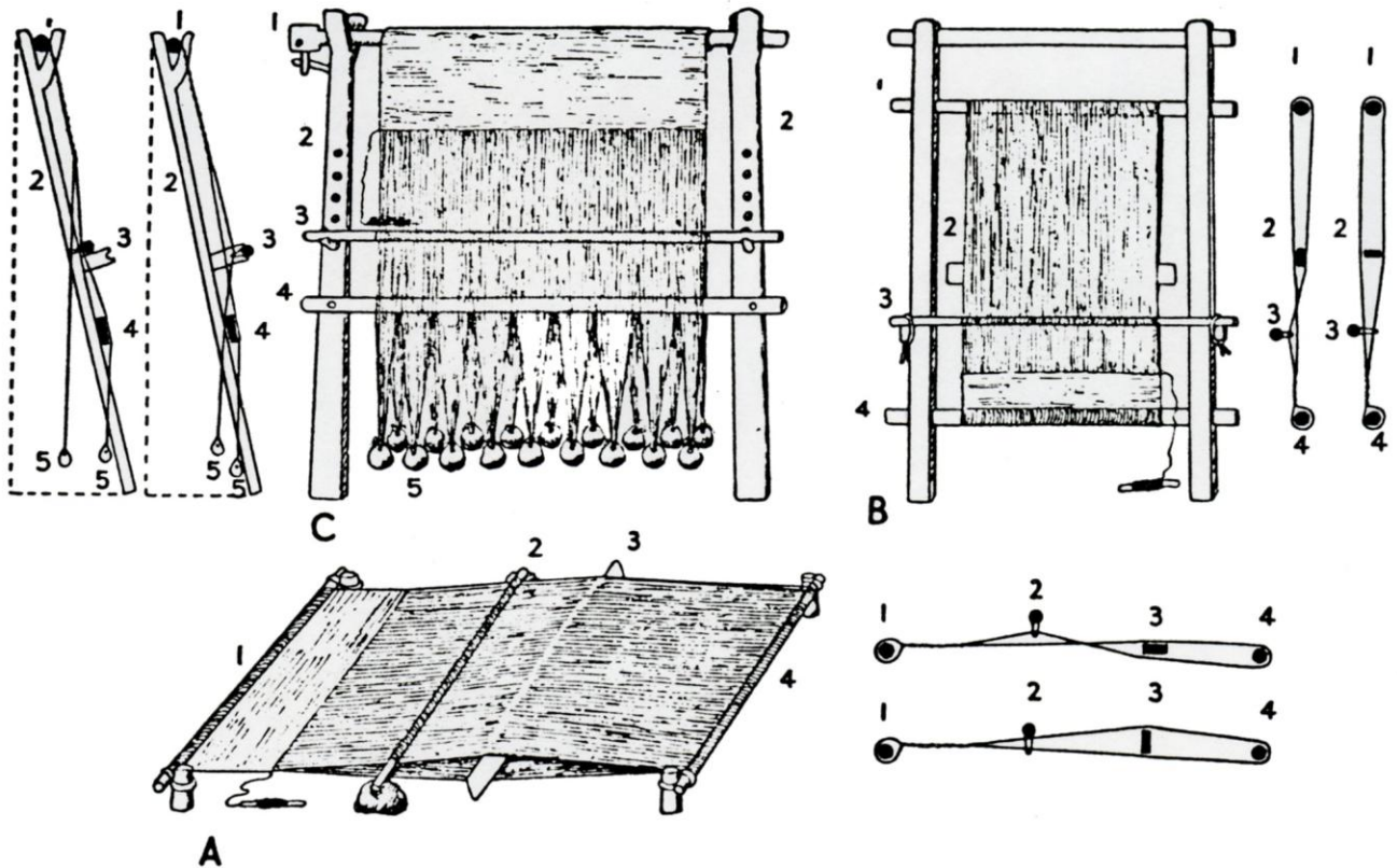
Fig. 32. Looms: (A) Horizontal ground-loom and shedding diagram: (1) breast-beam, (2) rod-heddle supported on stones, (3) shed-rod, (4) warp-beam. — (B) Vertical two-beamed loom and shedding diagram: (1) warp-beam, (2) shed-rod, (3) rod-heddle, (4) breast-beam. (C) Warp-weighted loom and shedding diagram: (1) warp-beam (revolving) held by a spoke, (2) side beams, (3) rod-heddle, (4) shed-rod, (5) warp-weights. — (D) Diagram to show (a) warp-threads, (b) shed-rod, and (c) rod-heddle with continuous spiral lashing. (Courtesy Editors of History of Technology.)
