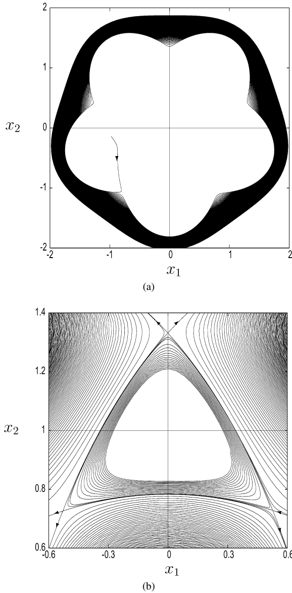
Fig. 3. The phase portraits of system (13) showing no large limit cycles near the critical point: a_{0c} = -0.0009467841 , b_{0c} = -1.8031893351 , a_{1c} = 0.0004961271 , b_{1c} = 2.8938995276 , a_{2c} = -0.0000151567 , b_{2c} = -0.9619832881 , a_{3c} = 0.1287269044 , b_{3c} = 0.0004658137 , (a) trajectory divergent to infinity; and (b) breaking of heteroclinic orbits.
