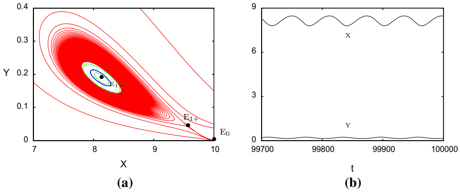
Fig. 10 Two limit cycles of system (5) for R_0 < 1 ( A > BC ) with A = 0.06085981 , B = 0.09375 , C = 0.20023941 and D = 0.1 , showing a tristable phenomenon: a phase portrait with the red/blue and green color curves denoting the simulations and estimates from the normal form (with amplitude r_1 \approx 0.1003 and r_2 \approx 0.3081 ), respectively; and b time history of the stable (outer) limit cycle (Color figure online)
