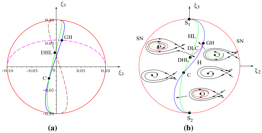
Fig. 19 Bifurcation curves for the codimension-3 BT bifurcation based on the normal form (86), displayed in the intersection of the cone and the 2-sphere \xi_1^2 + \xi_2^2 + \xi_3^2 = \sigma^2 , with red color for saddle-node, blue for Hopf and green for homoclinic, respectively: a with D = 0.2499 and \sigma = 0.1 , where the intersection point of the pink and blue curves is the degenerate Hopf bifurcation, and the intersection point of the brown and green curves denotes the degenerate homoclinic loop bifurcation; and b a schematic bifurcation diagram for b_1 > 0 (i.e., a_3 > 0 ) (Color figure online)
