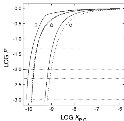
FIGURE 1: Effect of K_{p,G} on the goodness of fit obtained with Scheme 1. Equation 1 was fitted to data acquired at graded concentrations of [ ^3\text{H} ]NMS (a, no GMP-PNP; b, 0.1 mM GMP-PNP) or at 0.04 and 1.0 nM N -[ ^3\text{H} ]methylscopolamine and graded concentrations of carbachol (c, no GMP-PNP). The population of G proteins was assumed to be homogeneous (eq 2, n = 1 ). The parameter [S]_i/([R]_i + [S]_i) either was optimized (—) or was fixed at zero (---), and K_{p,G} was fixed at different values from <0.1 nM to 1 mM. The weighted sum of squares from the analysis at each value of K_{p,G} was compared with the asymptotic minimum to obtain the F statistic and the corresponding value of \log P plotted on the ordinate. Each relationship shown in the figure reflects six sets of data from three independent experiments; binding at graded concentrations of the radioligand was measured concurrently in the absence and presence of 0.01 mM unlabeled NMS (a, b), and binding at graded concentrations of carbachol was measured concurrently at both concentrations of the radioligand (c). In each analysis, single values of K_p , K_{p,G} , [R]_i/[G]_i , and [S]_i/([R]_i + [S]_i) were common to all six sets of data. The horizontal dotted lines indicate the 95%, 99%, 99.5%, and 99.9% levels of confidence. Values of \log K_{p,G} corresponding to 95% confidence are as follows for variable and fixed values of [S]_i/([R]_i + [S]_i) , respectively: a, -9.64 and -9.65 ; b, -9.84 and -9.83 ; c, -8.97 and -8.82 .
