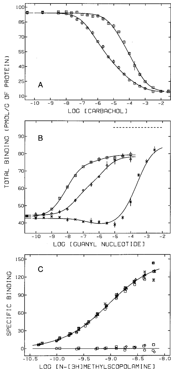
FIGURE 3: Fit of Scheme 1 to the binding of N -[ ^3H ]methylscopolamine, carbachol, and guanyl nucleotides in preparations of native membranes at high ionic strength. Total binding was measured following equilibration of the membranes in buffer B at graded concentrations of the ligand shown on the abscissa. Each panel contains the combined data from three experiments, and the conditions were as follows: (A) 1.02–1.14 nM [ ^3H ]NMS, no GMP-PNP (O), 0.1 mM GMP-PNP (□); (B) 1.01–1.09 nM [ ^3H ]NMS and 10 \mu M carbachol plus GMP-PNP (□), GTP \gamma S (◇), or GDP (⊗); (C) [ ^3H ]NMS alone (O, ◇, □) and plus 0.1 mM GMP-PNP (⊗, △, hourglass) (upper curve), [ ^3H ]NMS plus 0.01 mM unlabeled NMS (baseline). Different symbols in panel C denote data from different experiments (O, ⊗; ◇, △; □, hourglass). The dashed line in panel B indicates the binding of [ ^3H ]NMS in the absence of agonist and guanyl nucleotide ( 95.2 \pm 1.2 pmol/g of protein). The solid lines represent the best fit of the model ( n = 2 ) to the data taken together, and the parametric values are listed in Tables 4 and 5. Values plotted on the ordinate were obtained according to eq 6 in Chidiac et al. (1997), and the mean value of [P]_t used for panels A and B is 1.06 \pm 0.02 nM. Points shown at the lower and upper ends of the abscissa indicate binding in the absence of unlabeled ligand (A, B) and in the presence of 0.01 mM unlabeled NMS (A), respectively.
